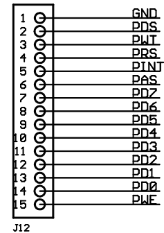
Parallel Port Test Point
