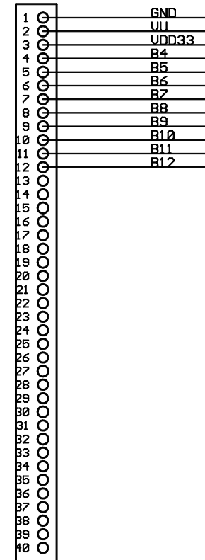
Connector F
