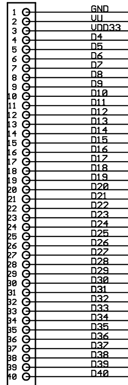
Connector D
