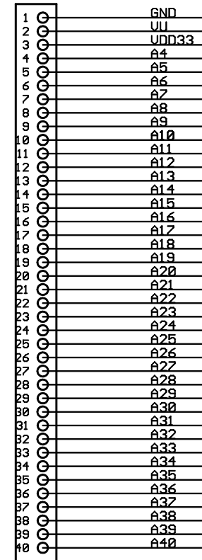
Connector E
