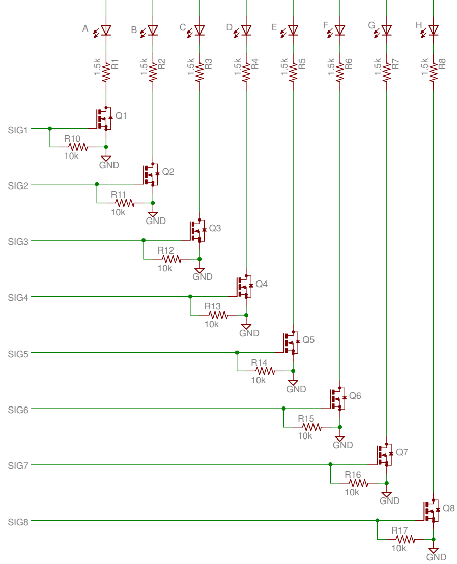
32MX7 Signal LEDs
