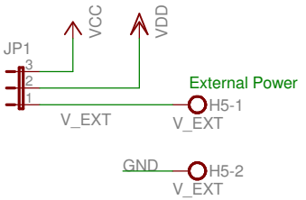
Power Select Jumper
