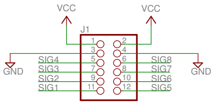
SM Board to 32MX7 Board Connector
